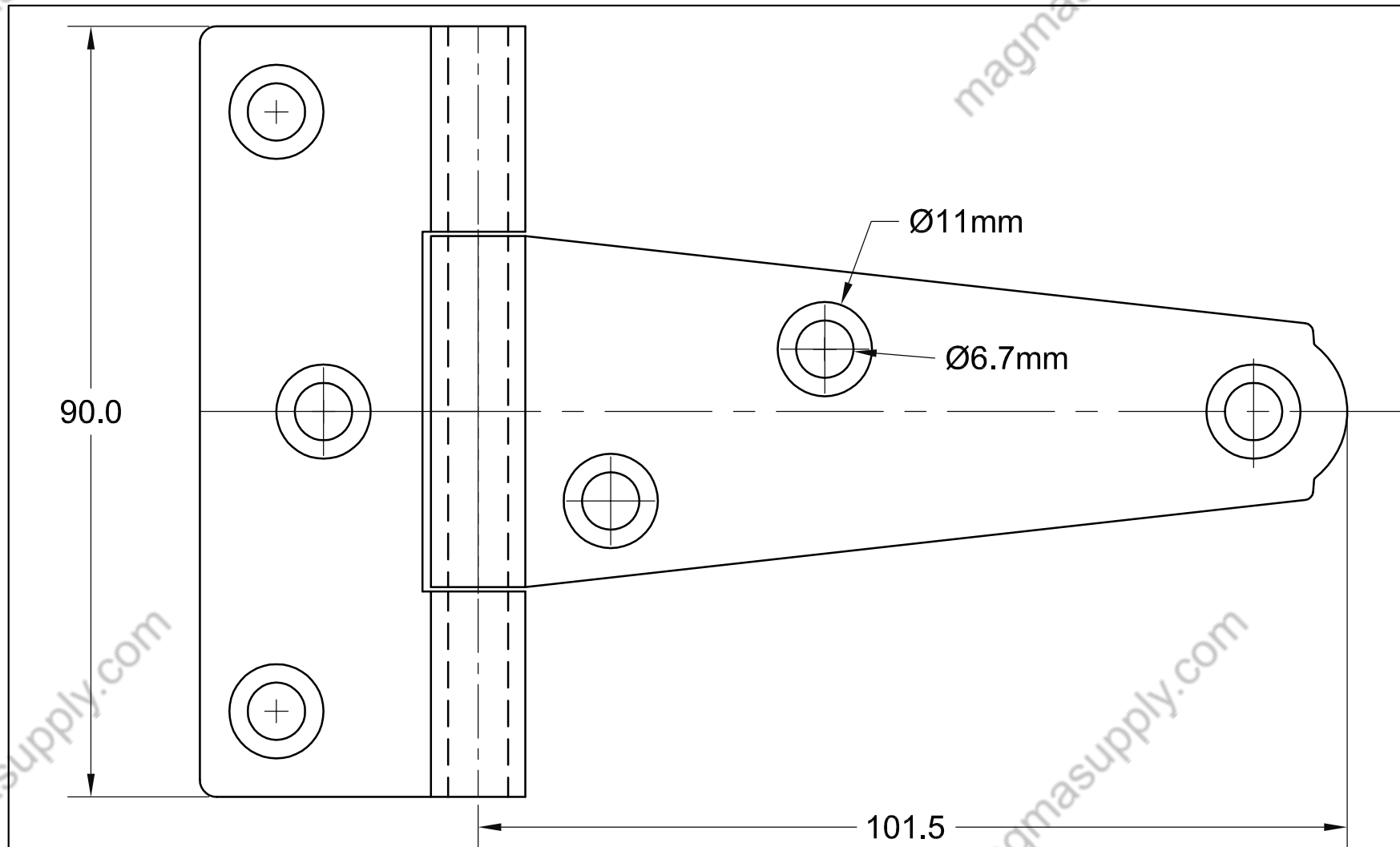
③ T HINGE ASSY 4"
